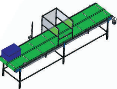
Auto Bin Feeding Conveyor Automation
