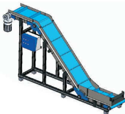
Inclined Modular Conveyor
